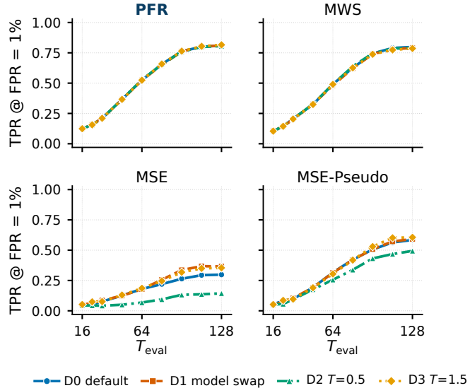
(b) Robustness to drafter substitution
