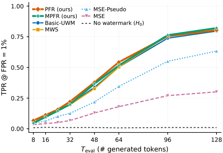
(a) Detection on the default drafter
